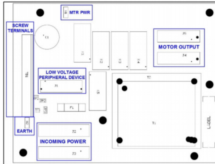
Figure 2 – Connector Layout
