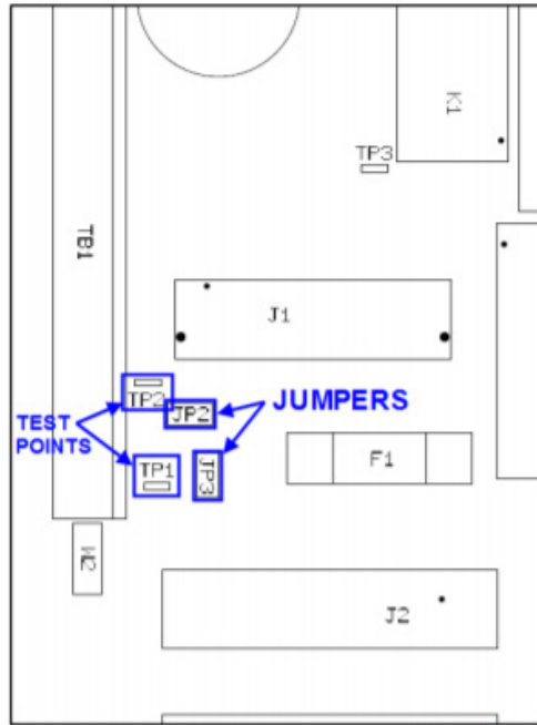
Figure F.2 - FRBii Jumpers and Test Points
